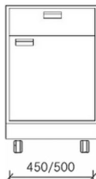
Combination of drawer and single door
